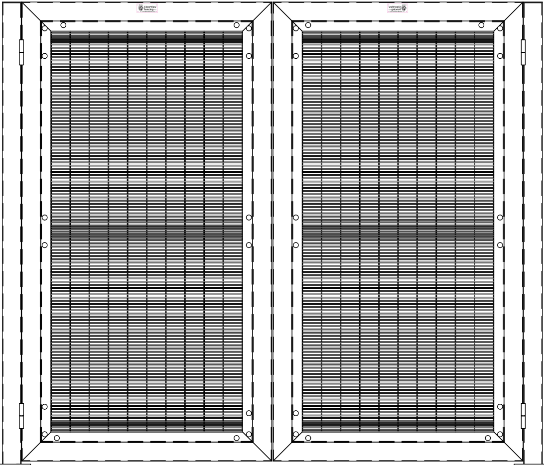
3 FRONT ELEVATION 1 : 15
