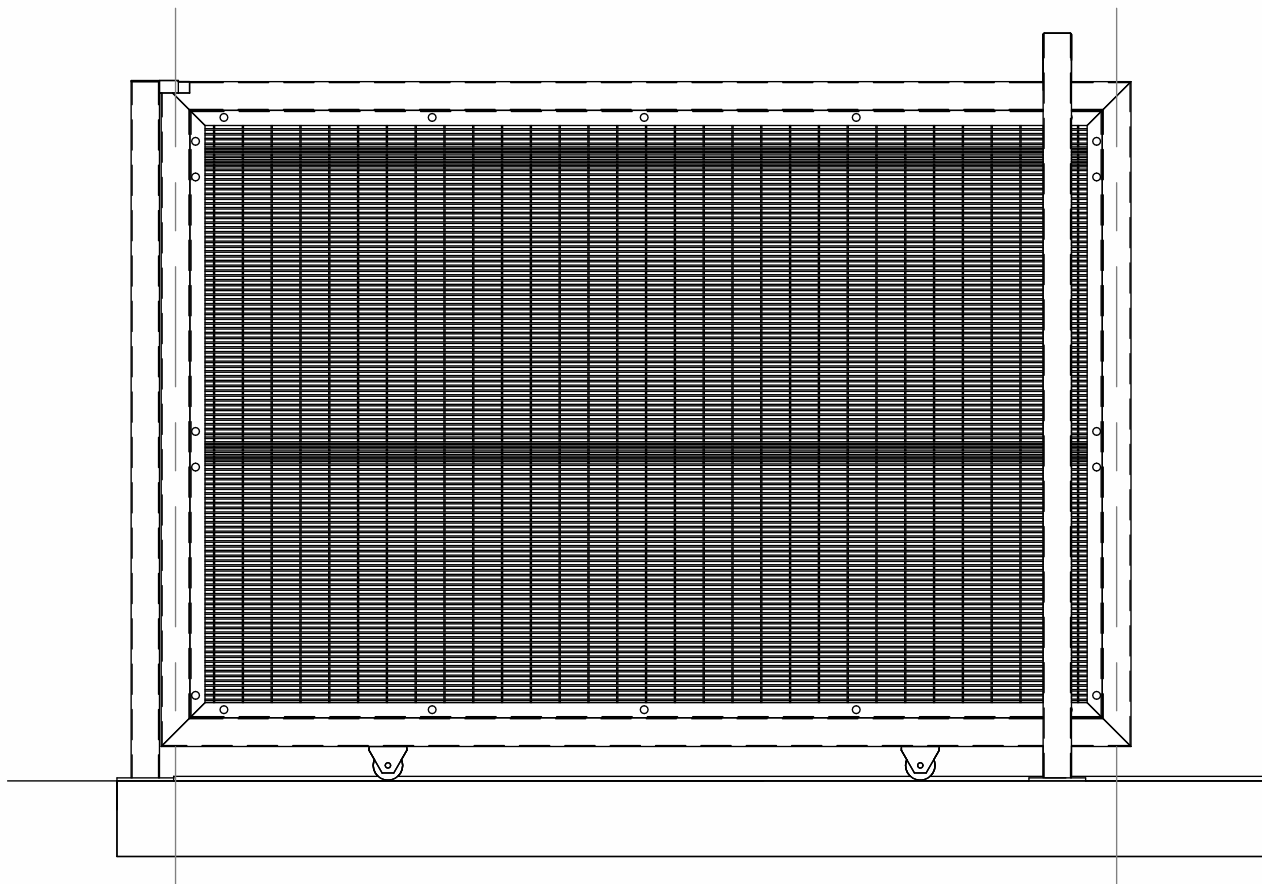
4 FRONT ELEVATION 1 : 20
